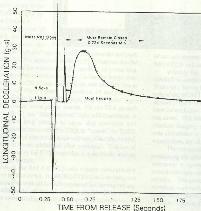
Figure 17. Functional Requirements for the Retard-sensing Rolamite, Minimum Parachute Retardation
